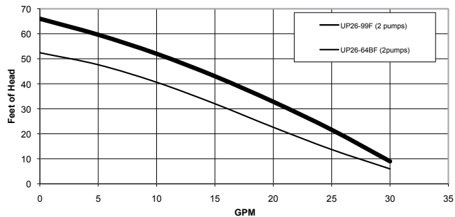
Two Pump Curve: UP26-64BF and UP26-99F
